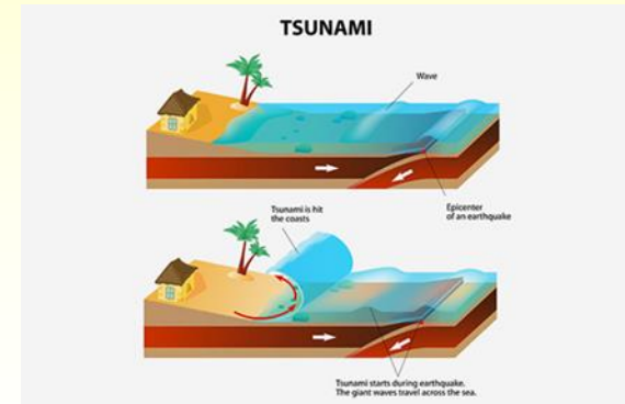
Tectonic Events
