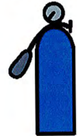
oxygen O 2
