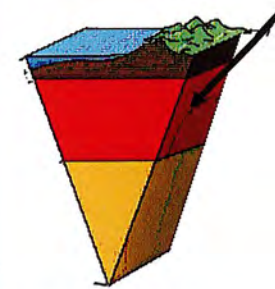
Mantle
