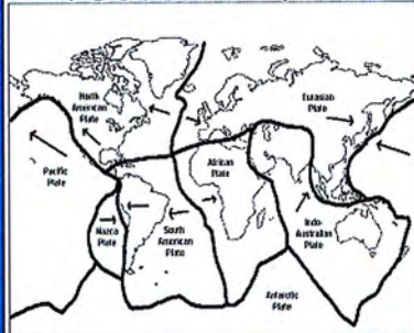
Tectonic Plates
